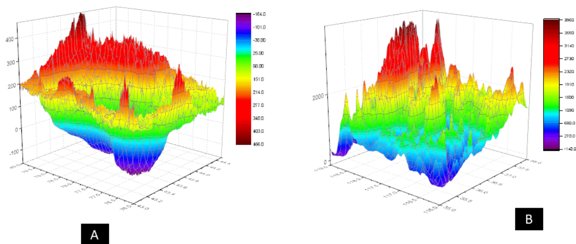
Figure 2. 3D Simulation of (a) FT-IR spectrum and (b) Raman spectrum of Brevetoxin (A)
