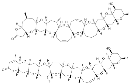
Molecular structure of Brevetoxin (A) (upper) and (B) (lower).
