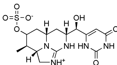
Molecular structure of Cylindrospermopsin.
