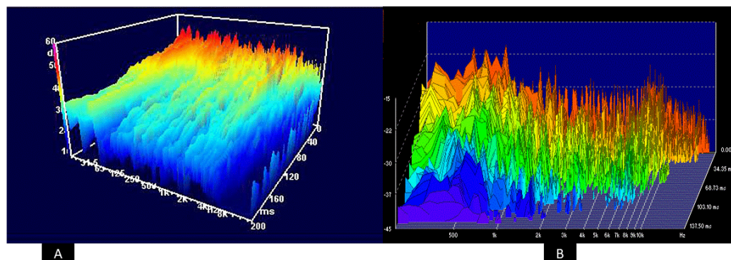
Figure 2. 3D Simulation of (a) FT-IR spectrum and (b) Raman spectrum of cylindrospermopsin
